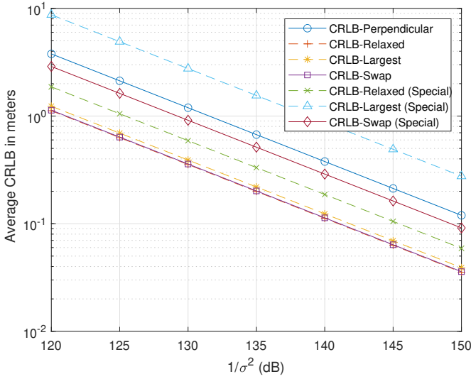
Fig. 4: Average CRLBs in meters in Case 1, when the receiver is close to the edge and \Delta = 10^\circ .
