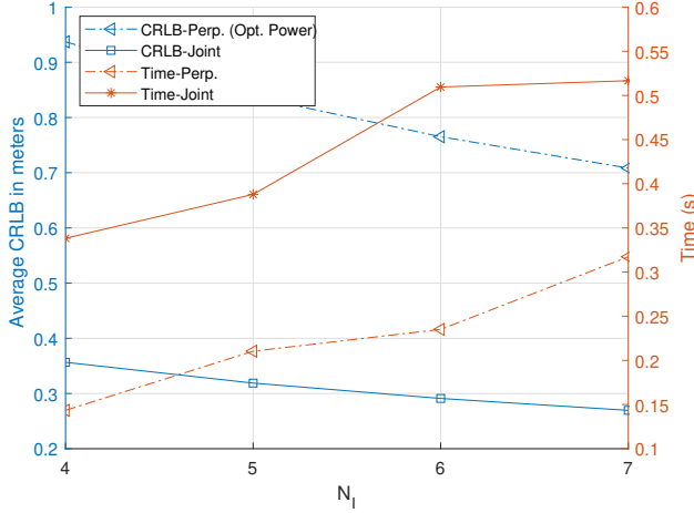
Fig. 11: Average CRLBs (in meters) and execution times of the proposed approach and the conventional approach (in which perpendicular LEDs are used in order and power optimization is performed) in Case 1, when the receiver is close to the edge, \Delta = 30^\circ , and 1/\sigma^2 = 130 dB.
