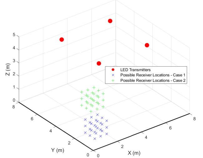
Fig. 2: VLP system configuration in the simulations. The center of grid is located at [1 \ 1 \ 1]^T m in Case 1 and at [3 \ 4 \ 1]^T m in Case 2.
