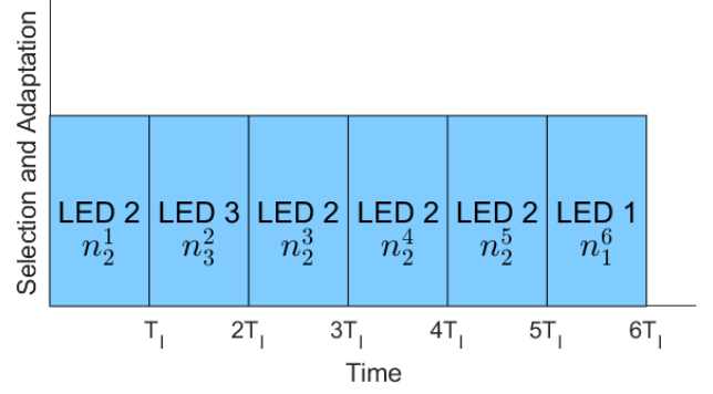
Fig. 1: An example of LED selection and orientation adaptation over N_I = 6 time intervals of duration T_I , using N_L = 4 LED transmitters, where the indices of the selected LED transmitters are given by s(1) = 2 , s(2) = 3 , s(3) = 2 , s(4) = 2 , s(5) = 2 , and s(6) = 1 . As will be illustrated in Section VI, it may be optimal not to employ all the LEDs (such as LED 4 in this example) during the localization process.
