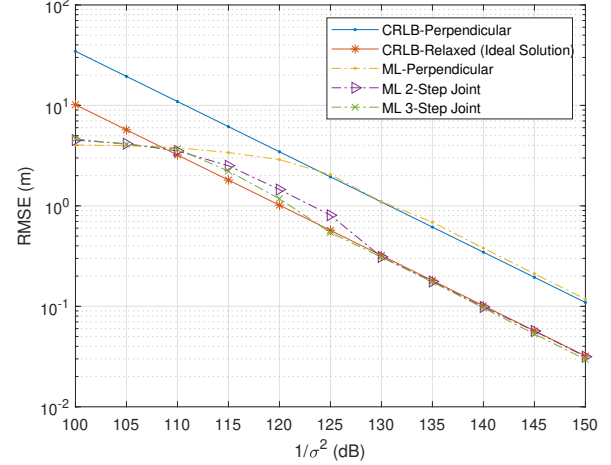
Fig. 12: RMSEs of the ML estimators in the multi-step algorithm together with the CRLBs (in meters) for the initial (perpendicular) configuration and for the ideal case of known VLC receiver position. In this case, the VLC receiver is located at [1, 1, 1]^T m. and \Delta = 30^\circ .
