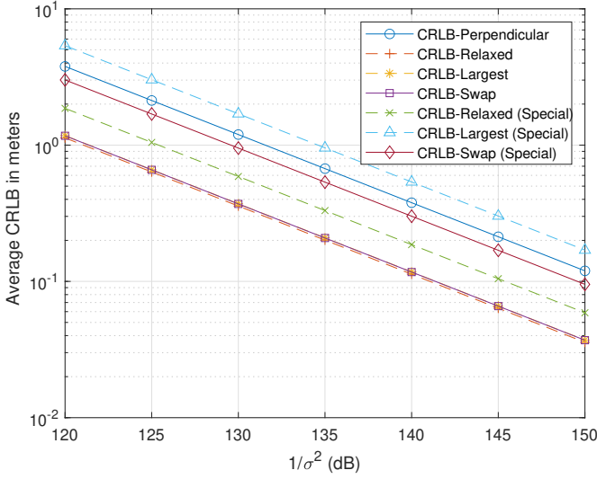
Fig. 3: Average CRLBs in meters in Case 1, when the receiver is close to the edge and \Delta = 30^\circ .
