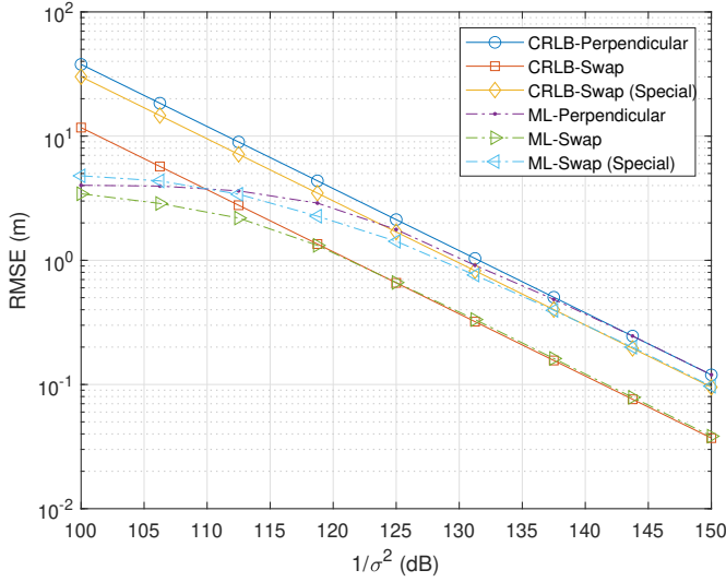
Fig. 7: RMSEs and average CRLBs in meters in Case 1, when the receiver is close to the edge and \Delta = 30^\circ .
